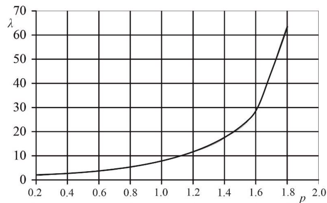
Figure 2 – Change in the logarithm of the coefficient \lambda = \lg \delta depending on the characteristic flow rate from the pipeline diameter when changing the parameter p
